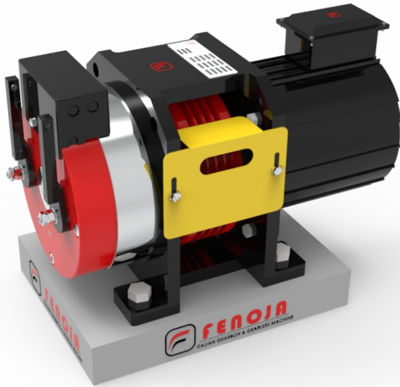
FENOJA250-1 Series Gearless Traction Machine Specification (Roping 2:1)
